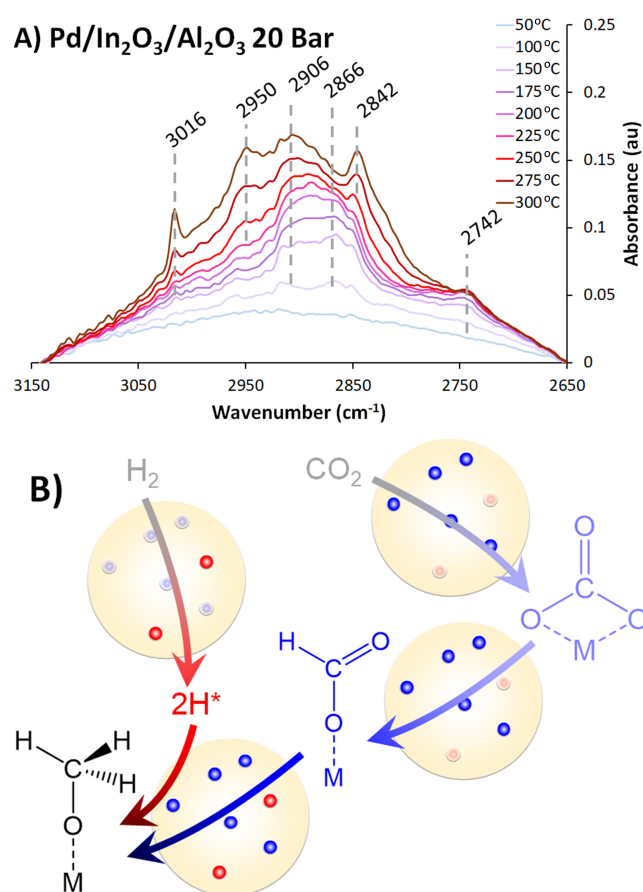
Figure 4. A) Operando DRIFTS difference spectra of Pd/In 2 O 3 /Al 2 O 3 , with 30 mL/min of 75 % H 2 and CO 2 , under 20 Bar of pressure and B) mechanistic implications with Pd represented as red circles, and In 2 O 3 as blue circles.
